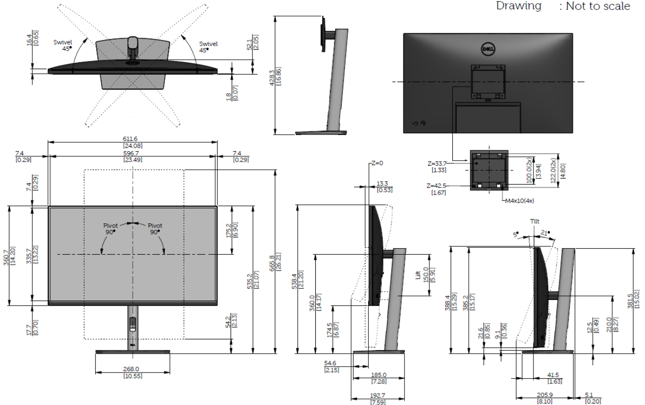
P2721Q Outline dimension
